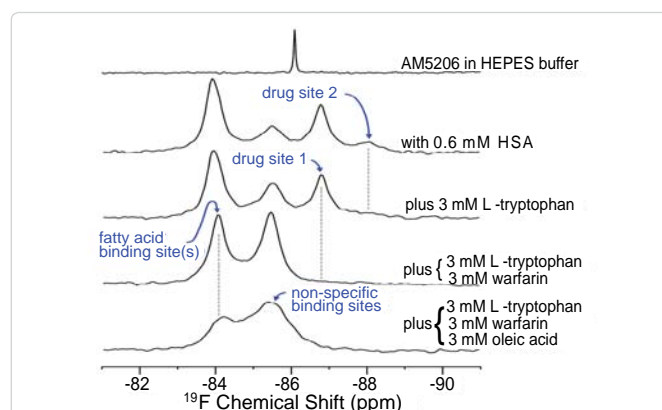
Figure 2: ^{19}\text{F} -NMR spectra of 0.6 mM AM5206, with 0.6 mM human serum albumin (HSA), and in the presence of one, two, or three of the competing site markers L-tryptophan, warfarin sodium and oleic acid.
