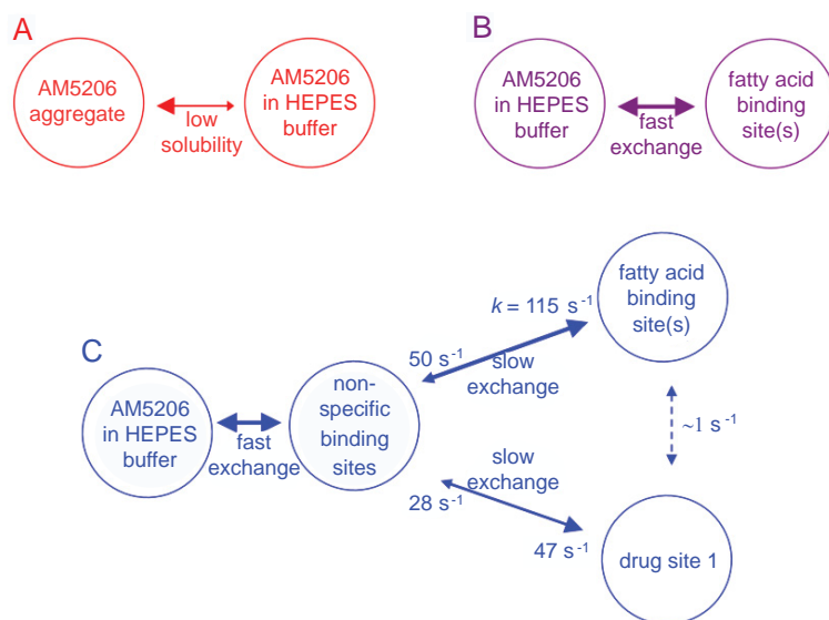
Figure 7: Proposed binding scenarios and the mechanism for the solubility enhancement by HSA: (A) In the aqueous buffer solution, AM5206 has a very low solubility ( \sim 70 \mu\text{M} ), and most of it forms aggregates or even precipitates. (B) With HSA present, a fast exchange allows AM5206 to rapidly bind to the fatty acid binding site(s) and to dissolve the aggregated/precipitated AM5206. (C) More binding sites (namely, drug site 1 and non-specific binding sites) on HSA become available at higher concentrations of AM5206. The exchange rate constants among these binding sites are indicated in the diagram.
