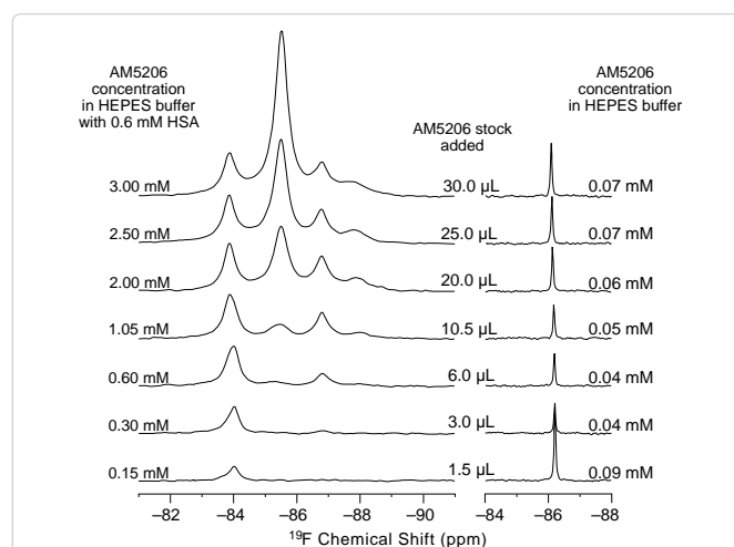
Figure 3: Left: ^{19}\text{F} -NMR titration experiments of AM5206 into 0.6 mM HSA solution. Right: ^{19}\text{F} -NMR spectra by adding the same amounts of AM5206 stock solution (50 mM in DMSO) into 500 \mu\text{L} HEPES buffer. The ligand concentrations listed in each spectrum reflect the soluble fraction of AM5206 as obtained by integrating the ^{19}\text{F} -NMR signals (cf. Figure 4).
